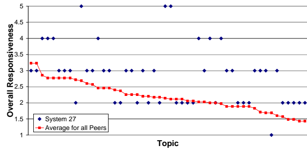
Figure 3: Overall Responsiveness vs. Mean.
